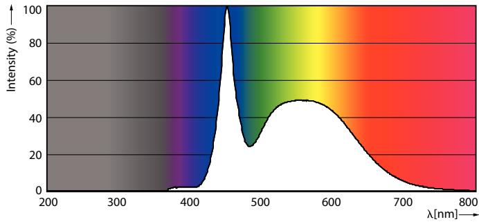
CorePro LEDbulb ND 17.5-150WA67E27 865FR
