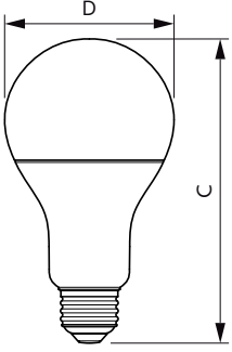
Bulb A67 220-240V 17.5-150W2500lm6500K
