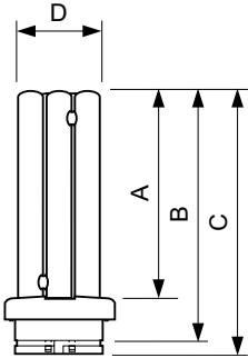
PL-R 14W/840/4P
