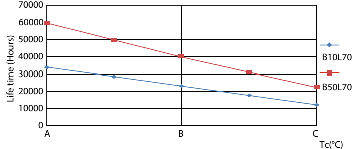
LEDtube_60K_LifetimeVsTc
