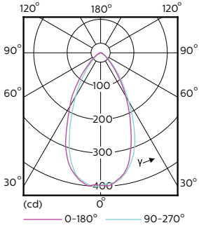
MASTER LEDspotMV 50W GU10 60D 355lm
