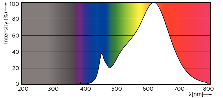
MASTER LEDspotMV 35W GU10 927 36D 260lm
